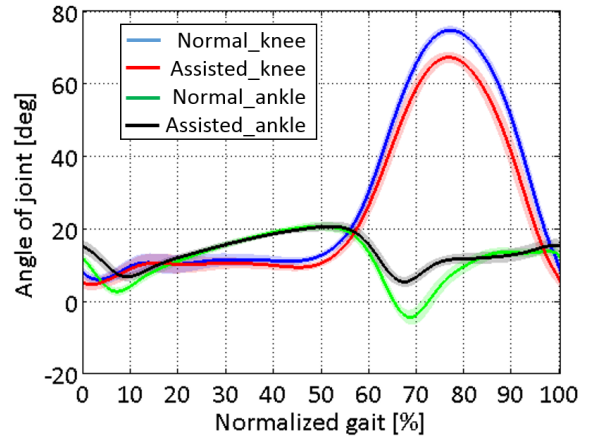
(a) Comparison of joint angles
