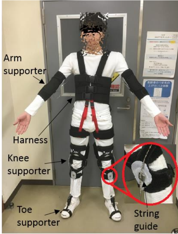
Fig. 1 Design of wearable assist device
