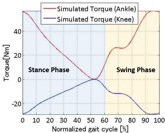
Fig. 6 Simulated joint torque (arm swing path)
