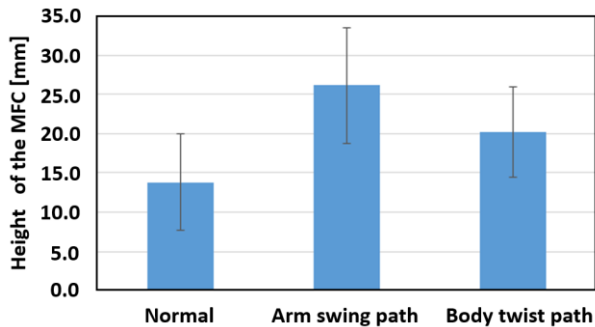
Fig. 10 Comparison of foot clearance
