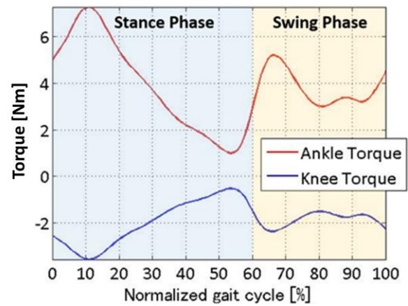
(b) Generated joint torque
