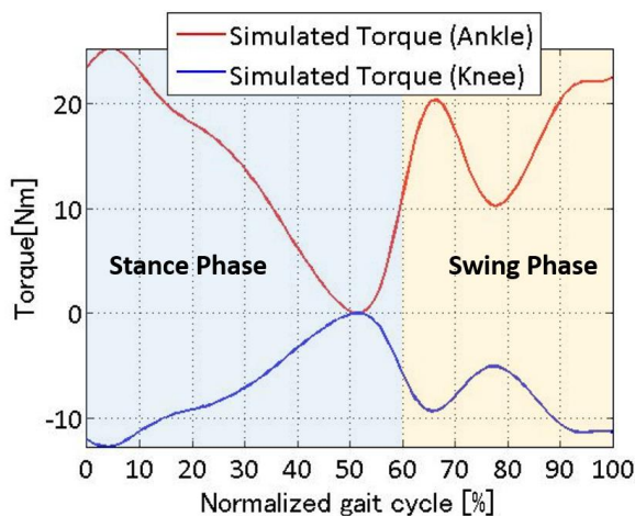
Fig. 7 Simulated joint torque (body twist path)
