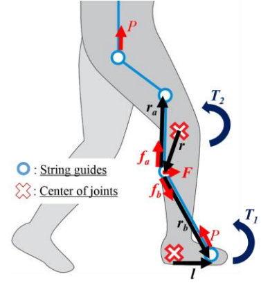
Fig. 2 Theory of generating resultant force and torque
